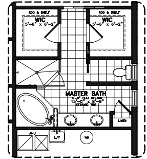
MASTER BATH OPTION 'B'
